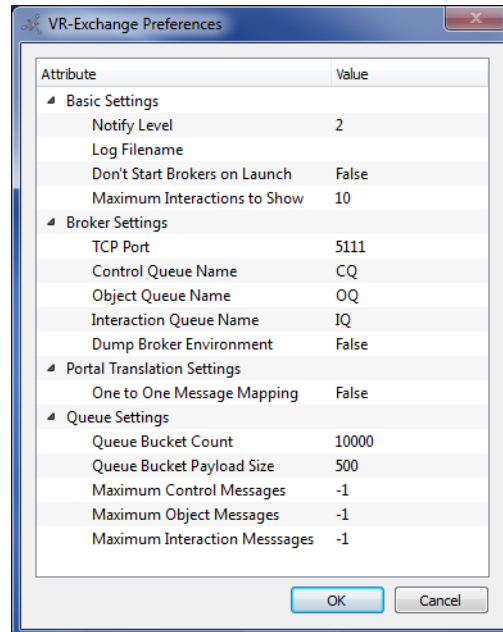
Figure 3-2. VR-Exchange Preferences dialog box
