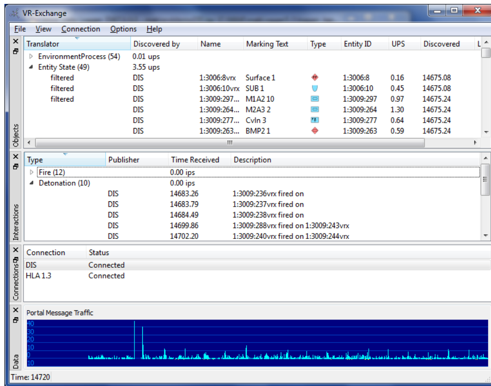
Figure 1-4. VR-Exchange Portal window
