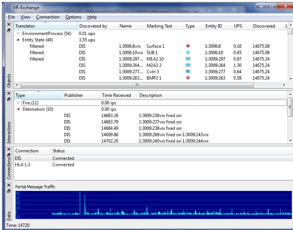
Figure 3-4. Object and interaction display
