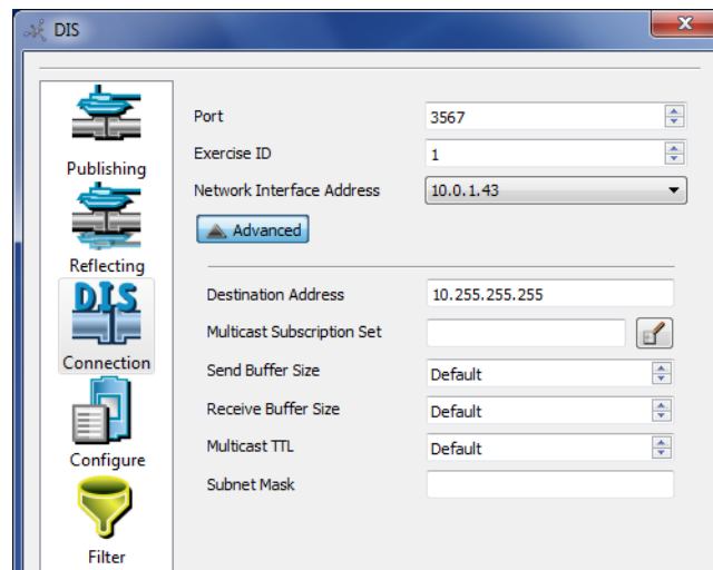
Figure 4-8. DIS Network Connections page
