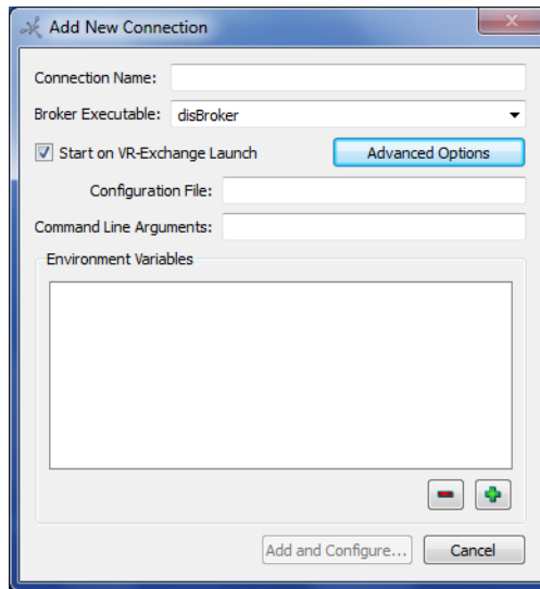
Figure 4-2. Add New Connection dialog box, Advanced Options
