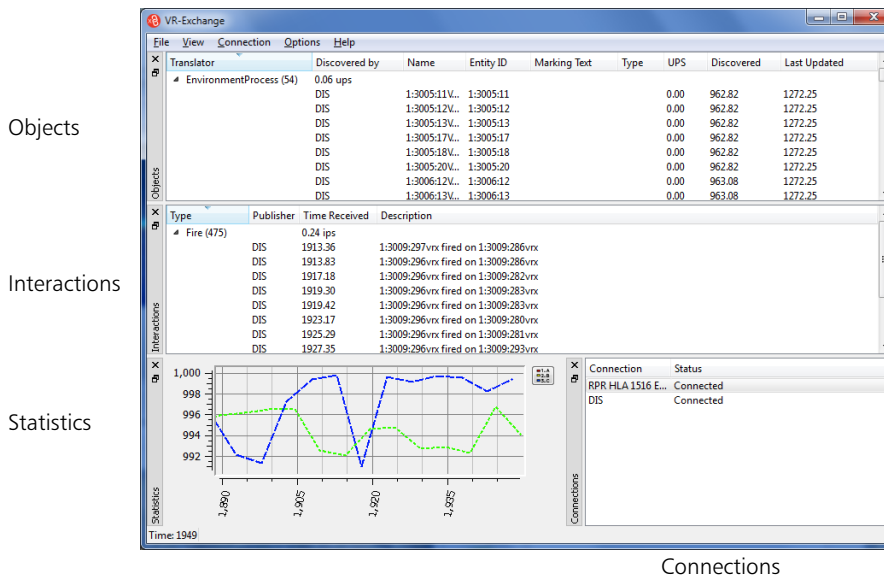
Figure 3-1. VR-Exchange Portal window
