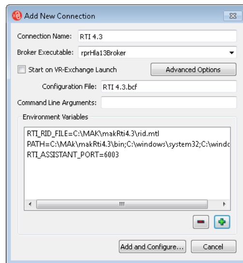
Figure 4-3. Environment variables
