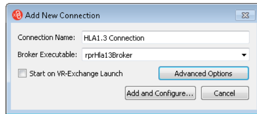
Figure 5-3. New connection
