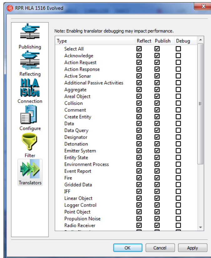
Figure 4-14. Translators page
