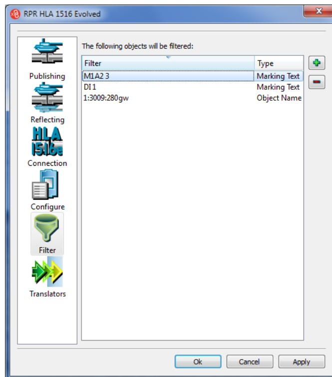
Figure 4-10. Filter page
