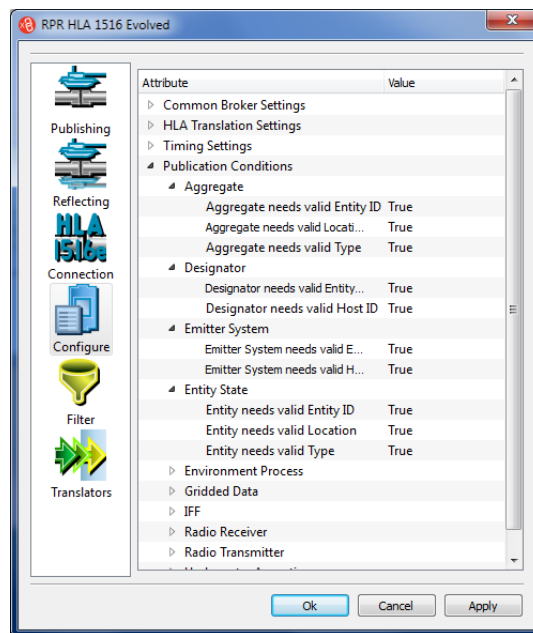
Figure 4-8. Publication conditions
