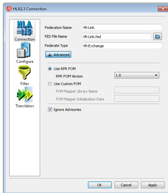
Figure 5-4. HLA connection
