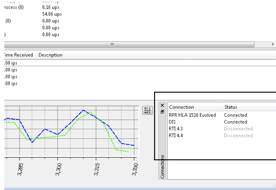
Figure 5-12. New brokers
