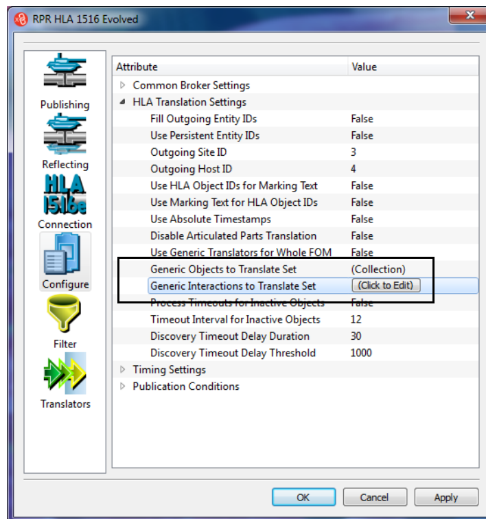
Figure 4-6. Collection value
