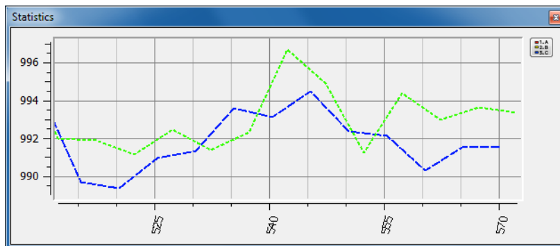
Figure 3-9. Statistics View
