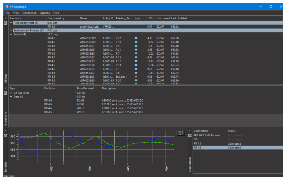
Figure 47. VR-Exchange routing RTI 4.5 traffic to RTI 4.6
