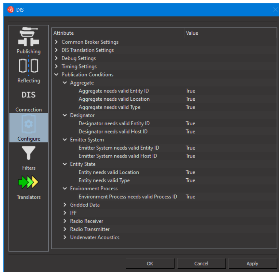
Figure 25. Publication conditions
