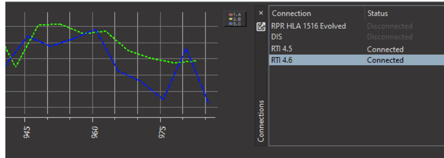
Figure 46. Connected brokers
