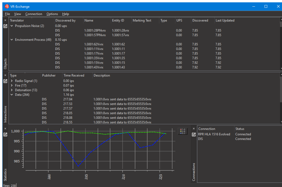
Figure 9. Object and interaction display
