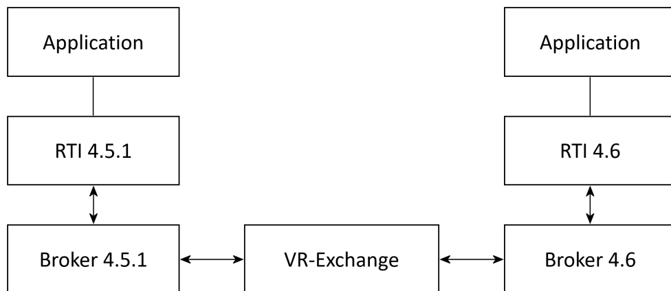
Figure 34. VR-Exchange configuration - one computer
