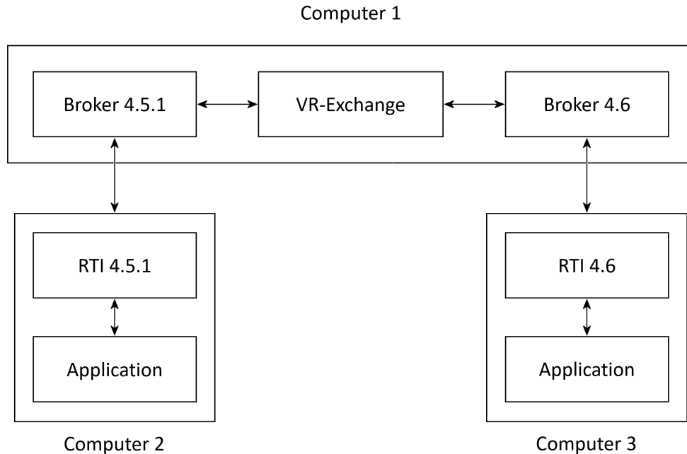
Figure 35. VR-Exchange configuration - three computers
