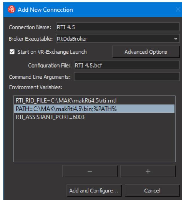
Figure 20. Environment variables
