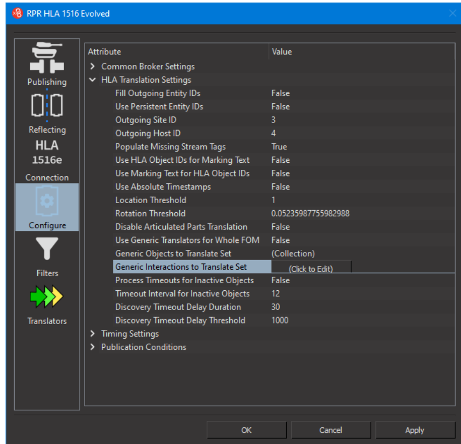
Figure 23. Collection value
