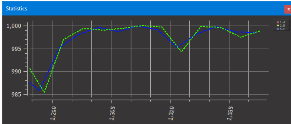
Figure 14. Statistics View
