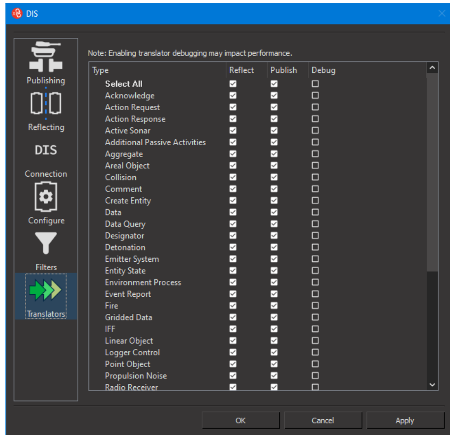
Figure 31. Translators page
