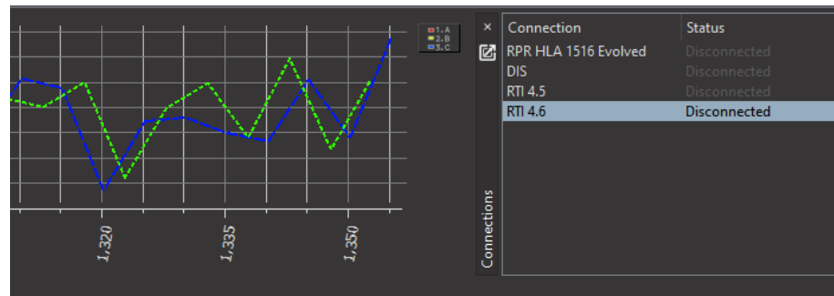
Figure 41. New brokers
