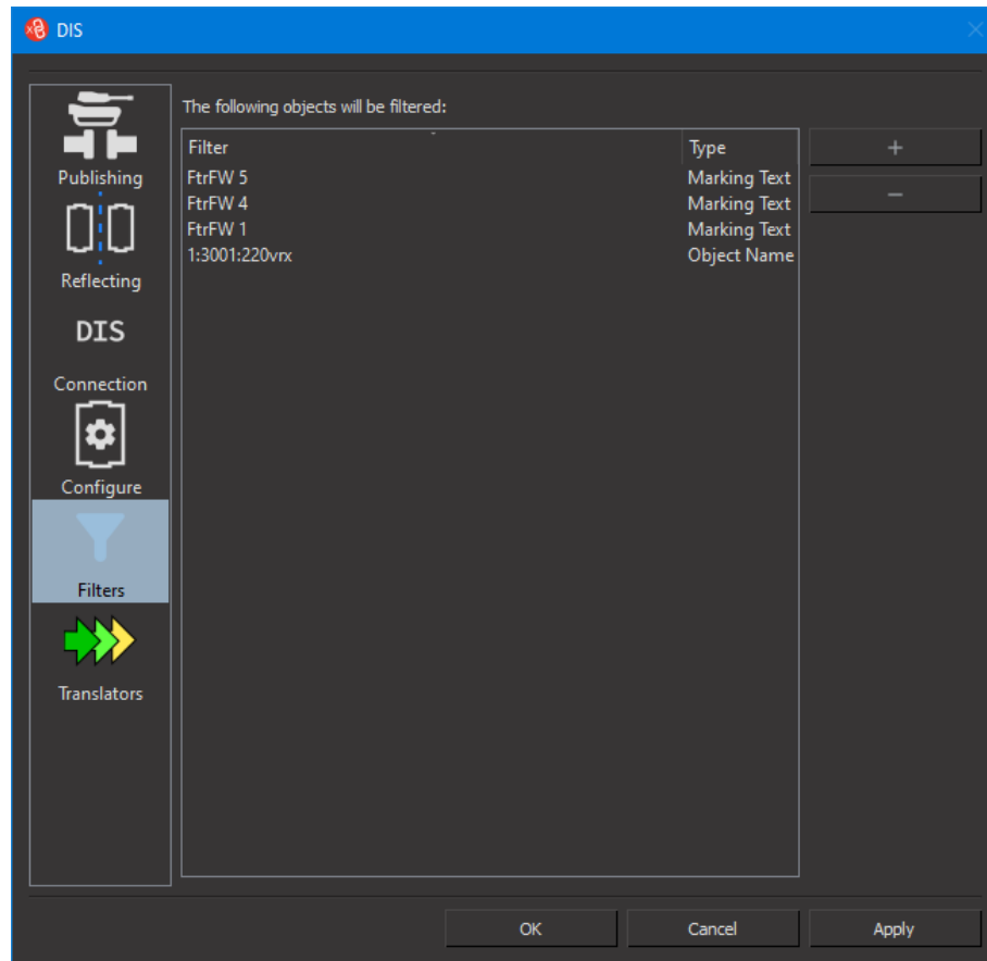
Figure 27. Filter page
