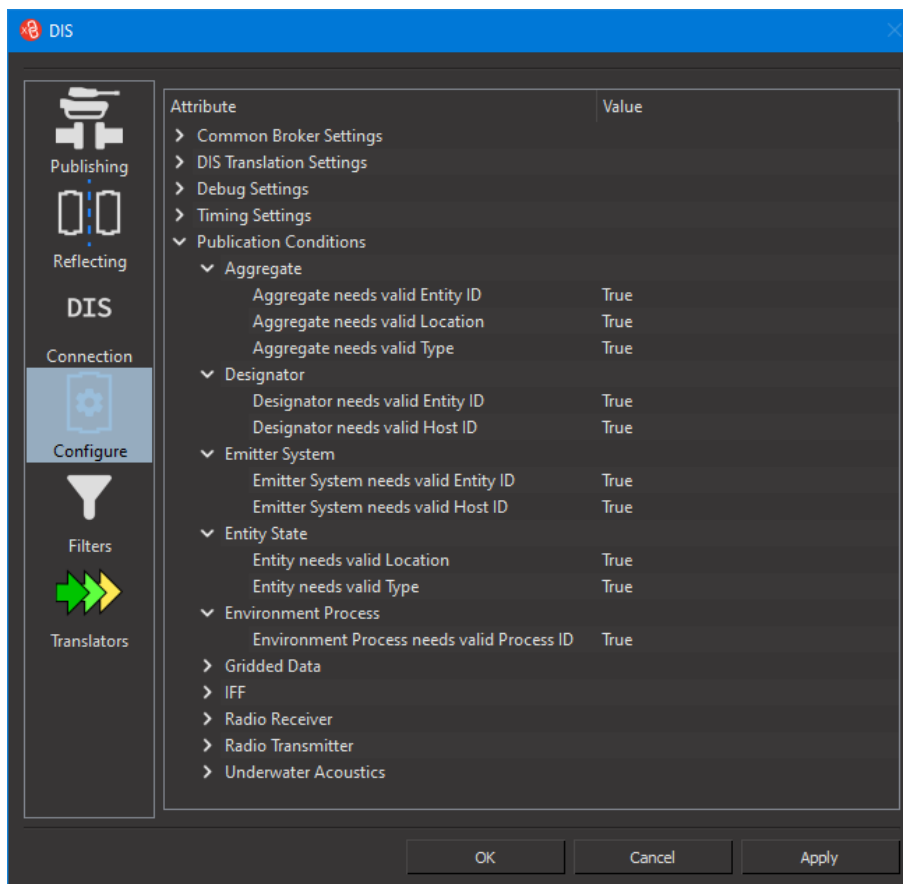
Figure 25. Publication conditions
