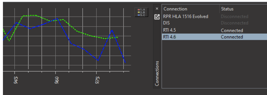
Figure 46. Connected brokers
