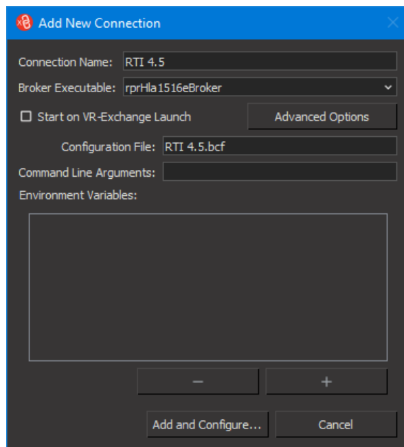
Figure 37. Add New Connection dialog box, Advanced Options
