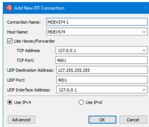
Figure 43. Add New RTI Connection
