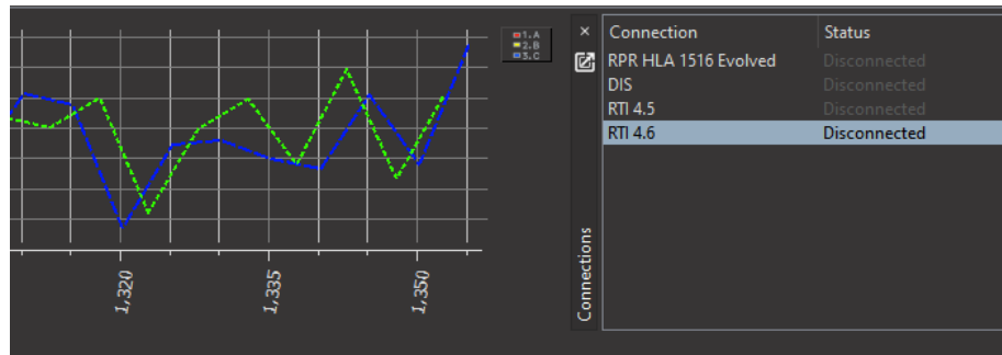
Figure 41. New brokers
