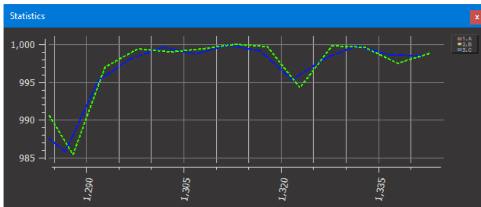
Figure 14. Statistics View
