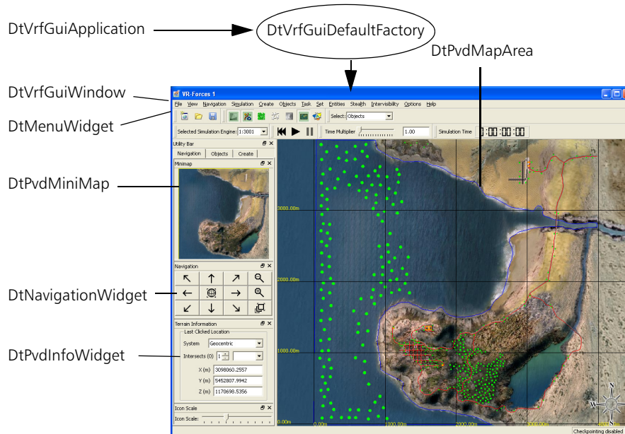
Figure 13-1. VR-Forces GUI Architecture
