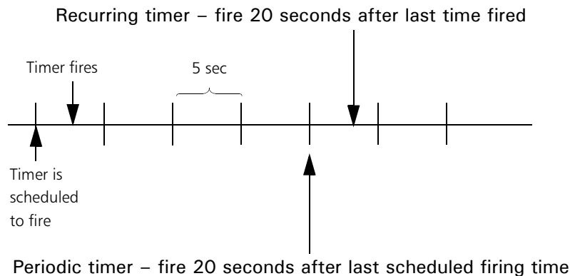
Figure 16-1. Recurring and periodic timers
