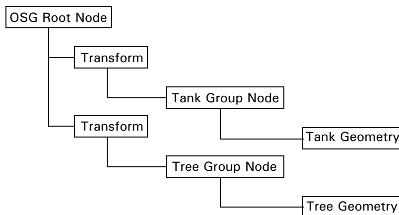
Figure 7-1. Scene graph
