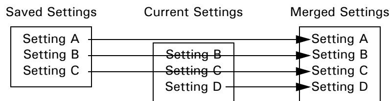
Figure 3-1. Merged settings
