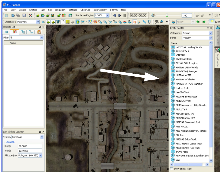
Figure 15. Entity Palette
