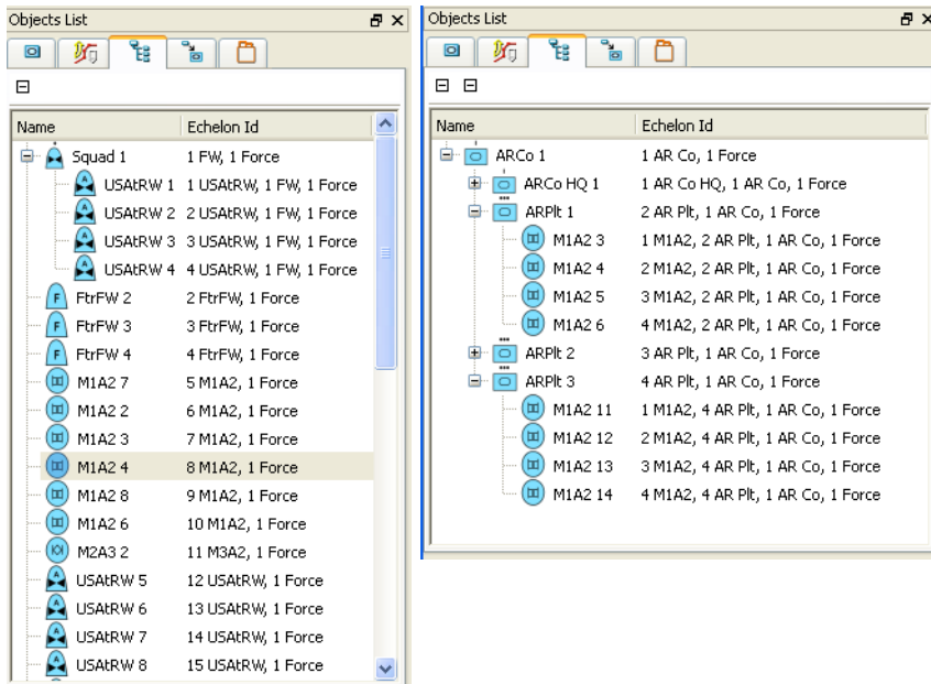
Figure 9. Echelon View
