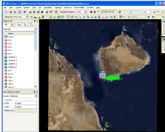
Figure 3. maklandDemo scenario
