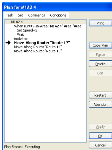
Figure 8. Entity plan
