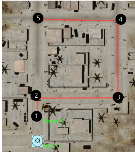
Figure 17. Vertex locations
