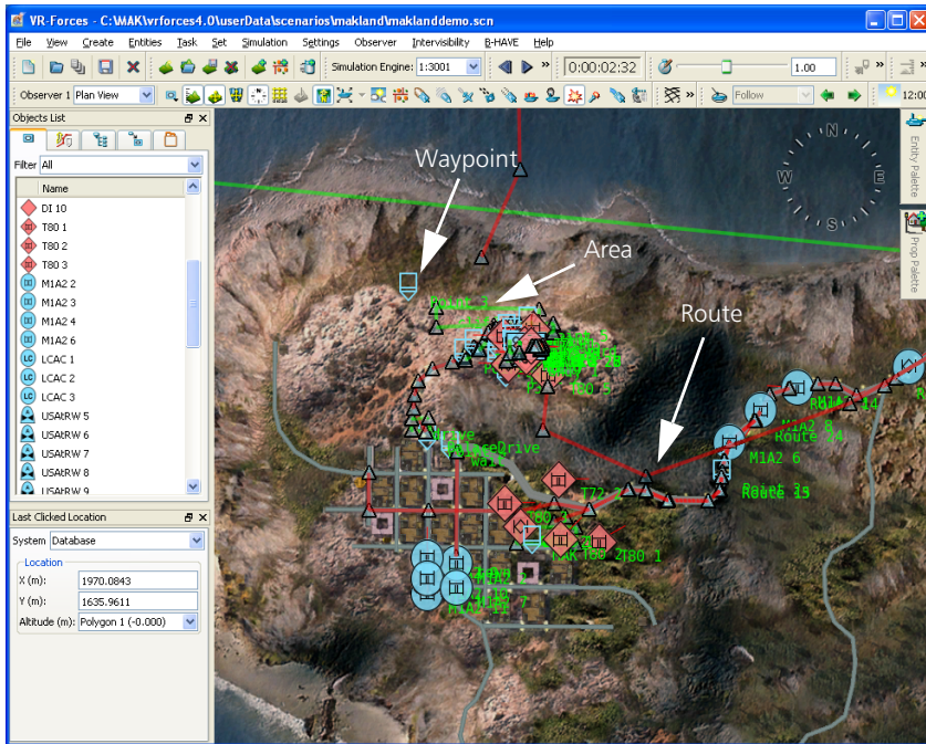
Figure 10. Tactical graphics
