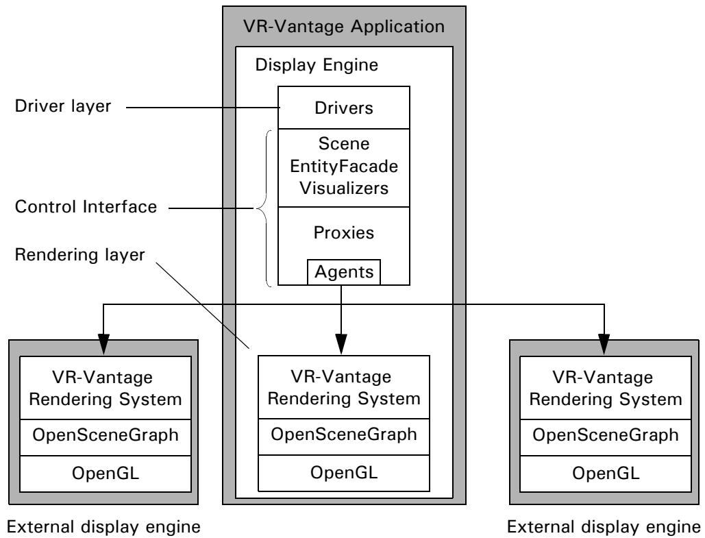
Figure 2-1. VR-Forces GUI architecture
