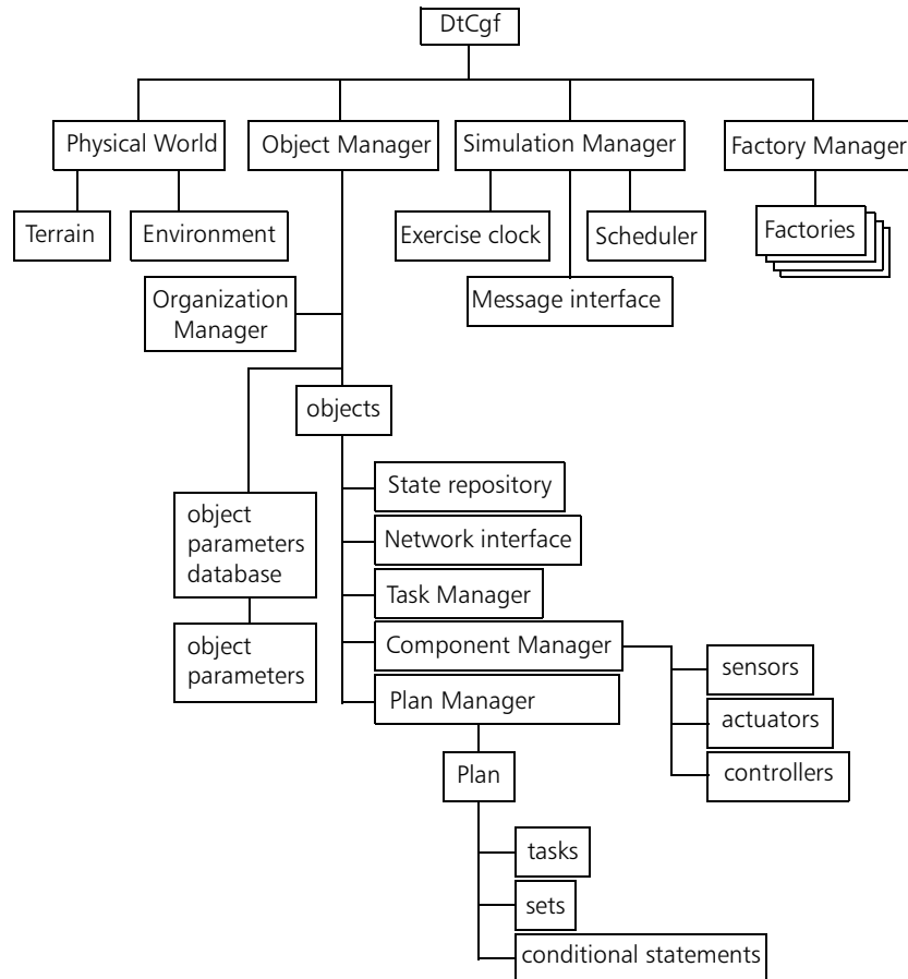
Figure 2-1. VR-Forces architecture
