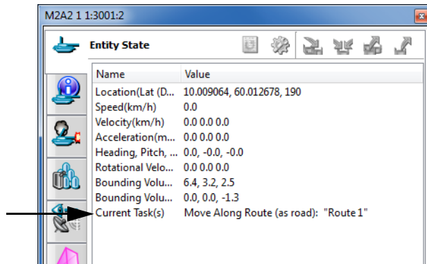
Figure 21. Entity Information dialog box
