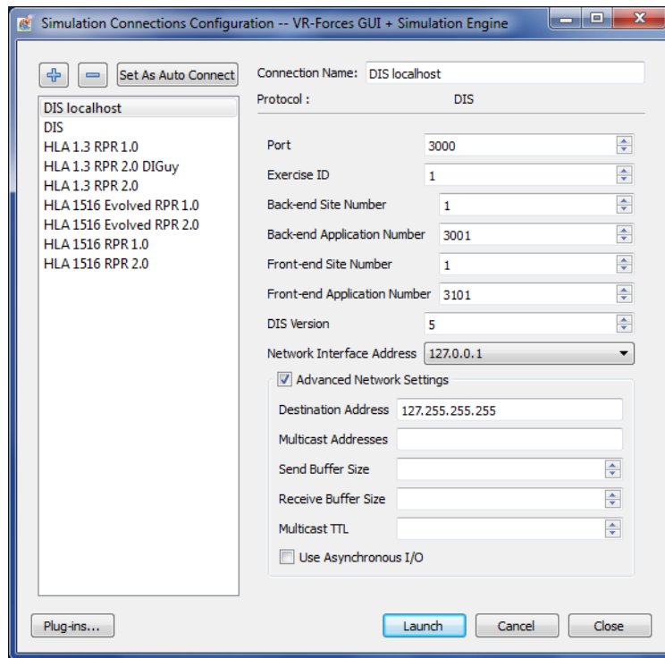
Figure 1. Simulation Connections Configuration dialog box
