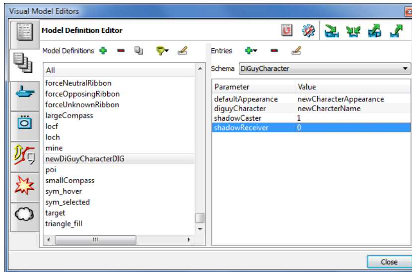
Figure 4. DI-Guy character parameters
