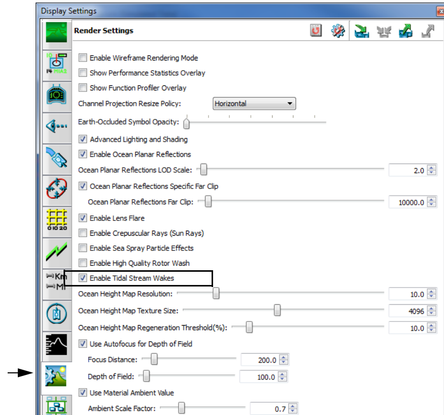
Figure 15-9. Render Settings page
