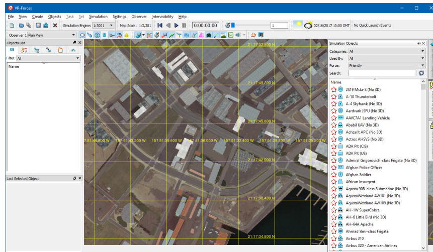
Figure 1-15. Entities Palette
