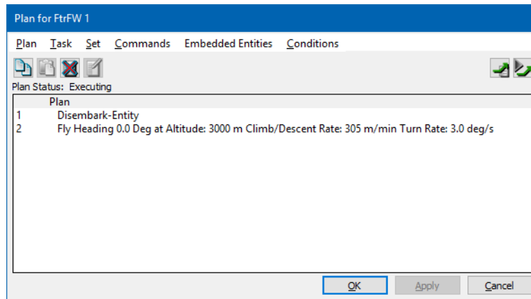
Figure 1-7. Plan window
