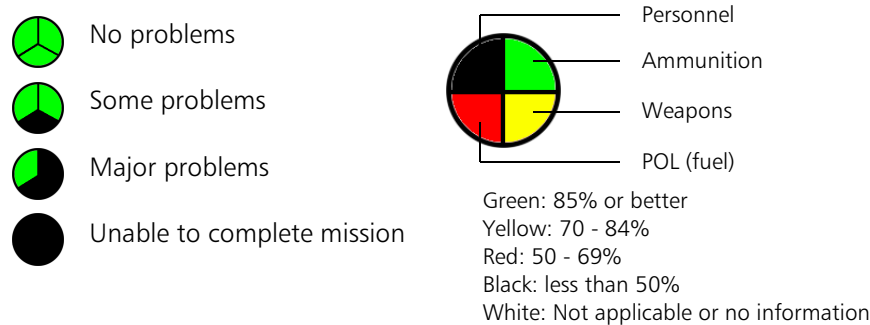
Figure 1-41. Gumball charts
