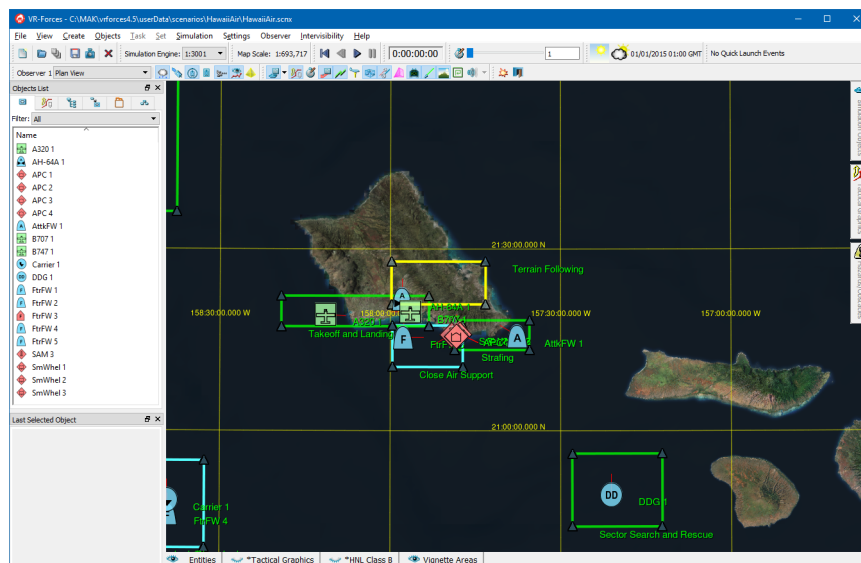
Figure 1-5. MaklandCoordinatedAttack scenario
