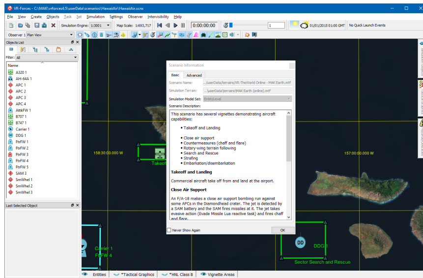
Figure 1-4. Scenario information
