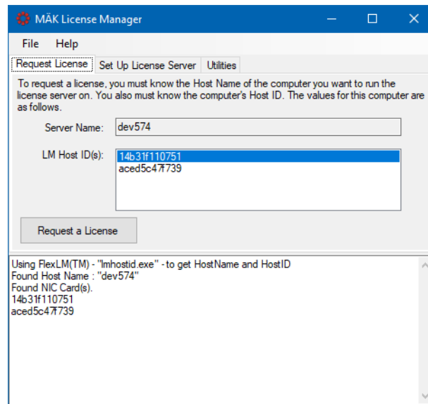
Figure 5-4. License Manager
