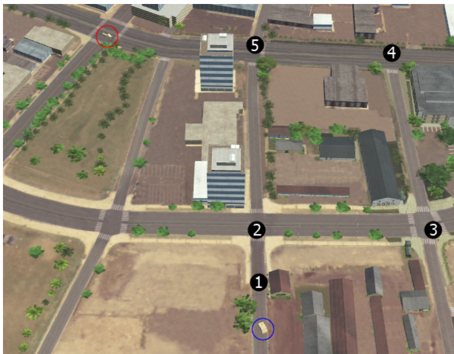
Figure 32. Vertex locations
