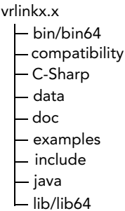
Figure 2-1. VR-Link directory structure
