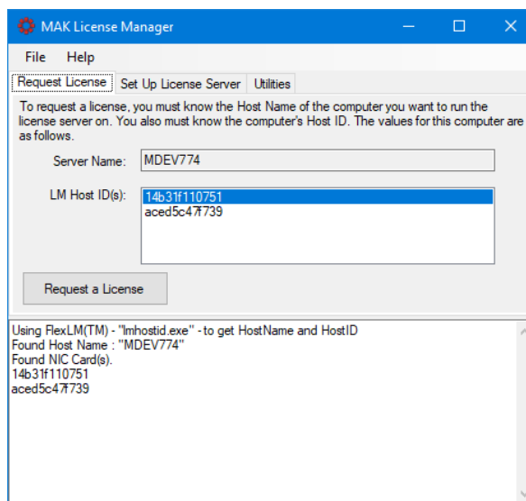
Figure 11. License Manager
