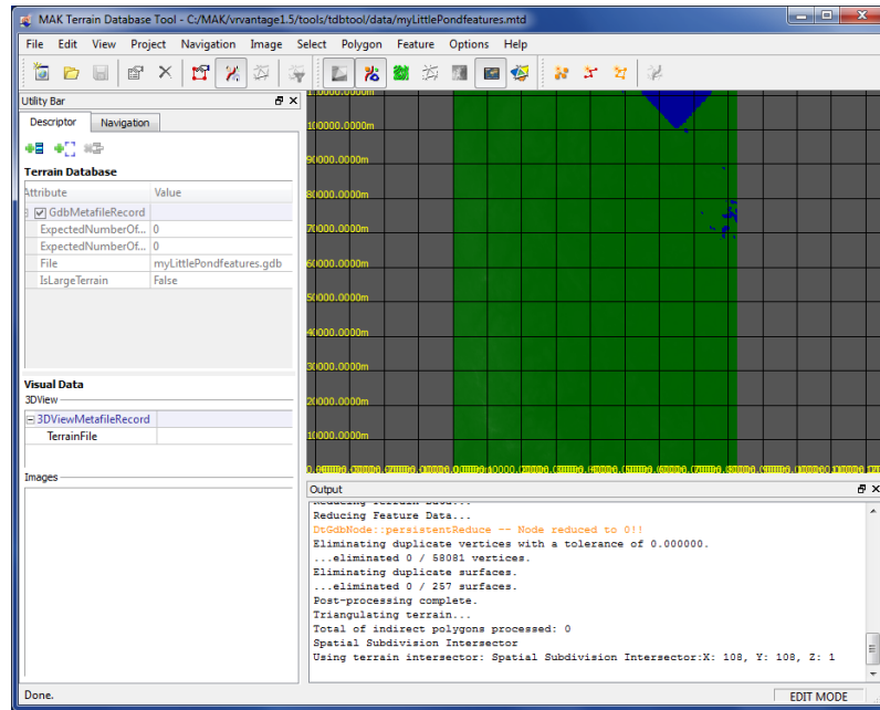
Figure 4-30. New terrain
