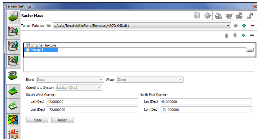
Figure 4-6. New image
