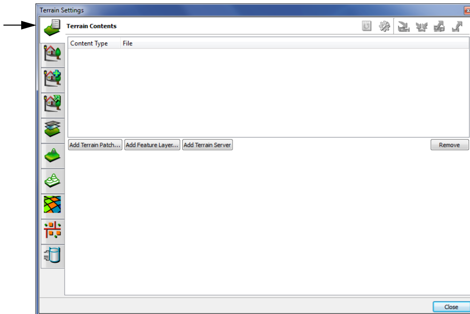
Figure 3-9. Terrain Contents
