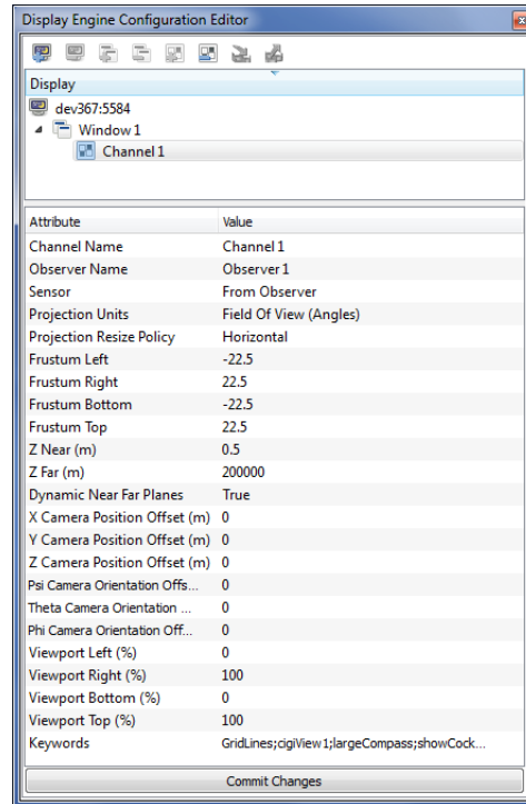
Figure 1-4. Channel attributes
