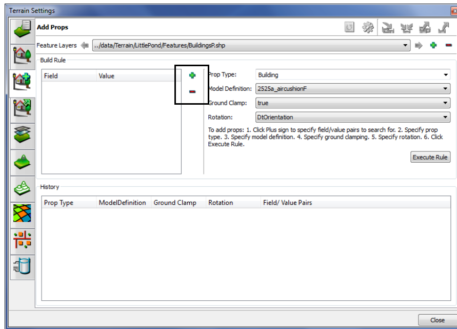
Figure 4-11. Add build rule
