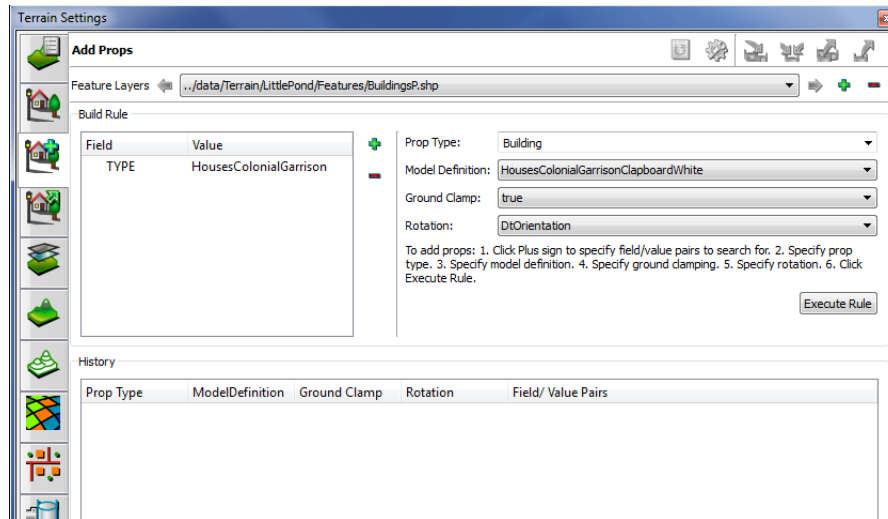
Figure 4-13. Completed rule
