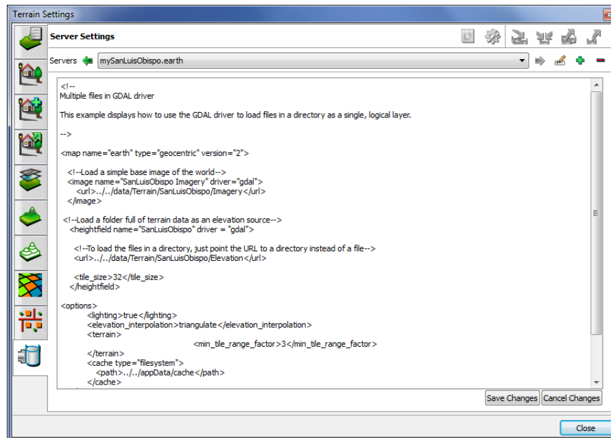
Figure 4-19. mySanLuisObispo.earth server
