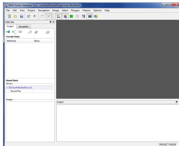
Figure 4-28. New project
