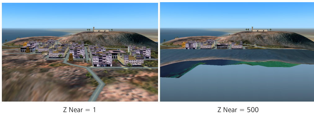
Figure 1-5. Near clipping
