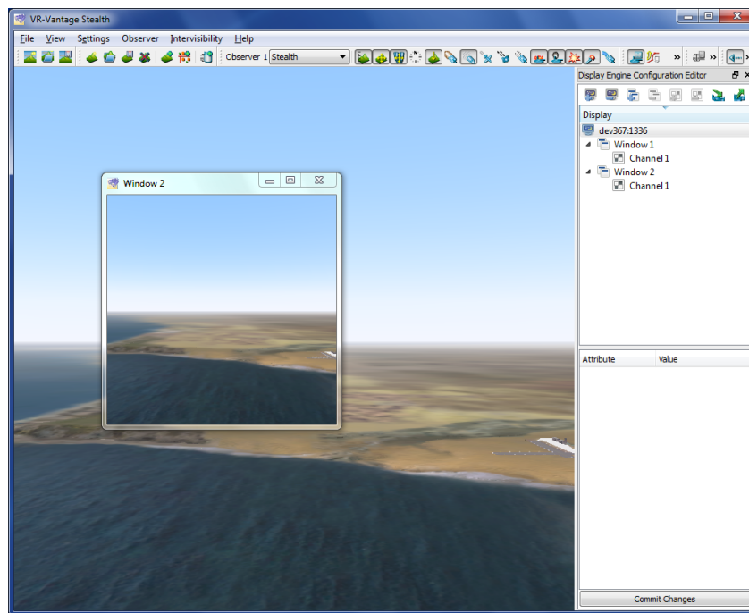
Figure 1-1. New window
