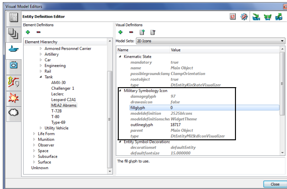
Figure 6-15. Military Symbol Icon Visualizer
