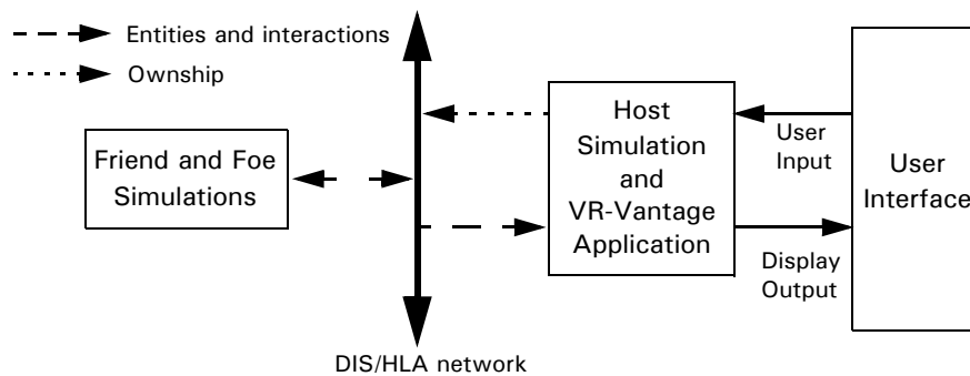
Figure 11-10. Integrated Visual/Simulation Application Configuration
