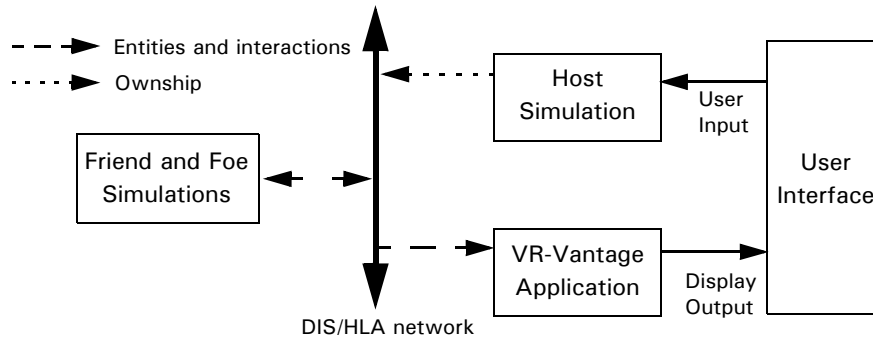
Figure 11-9. Distributed Visual/Simulation Application IG Configuration
