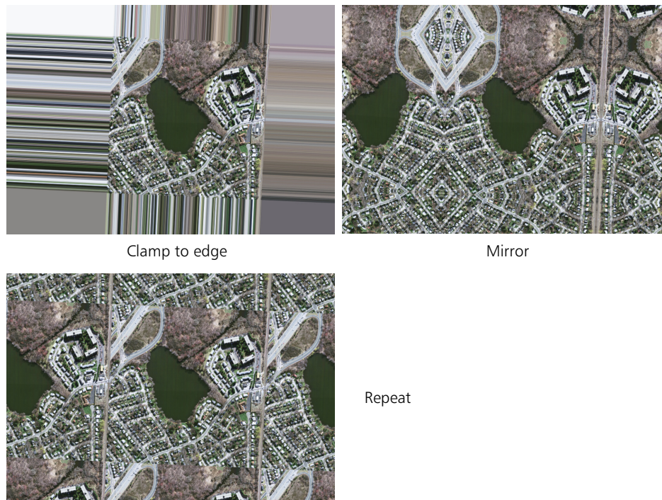
Figure 3-5. Raster image wrap effects (Clamp to Edge, Mirror, Repeat)
