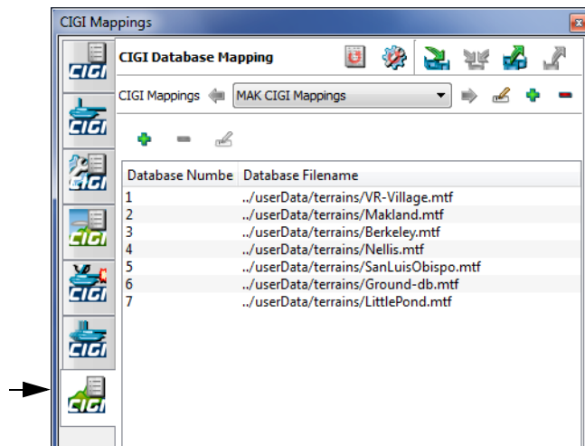
Figure 11-5. CIGI Database Mappings page
