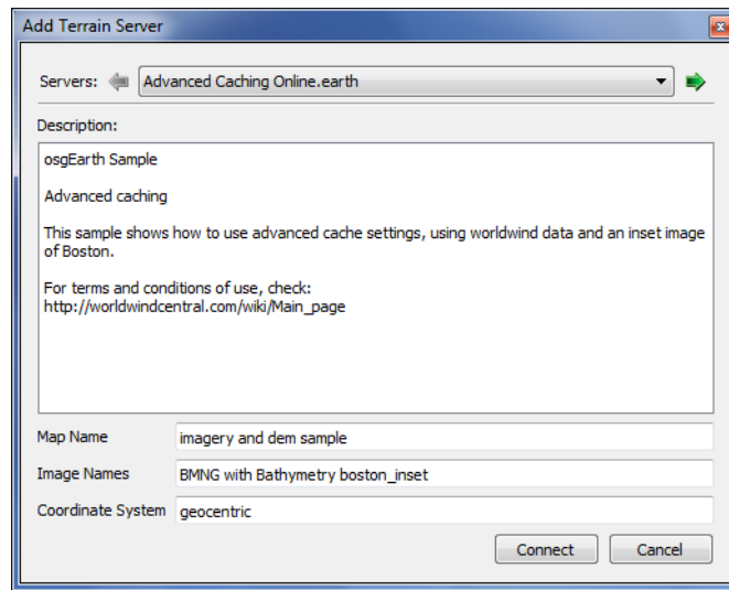
Figure 3-16. Add Terrain Server dialog box
