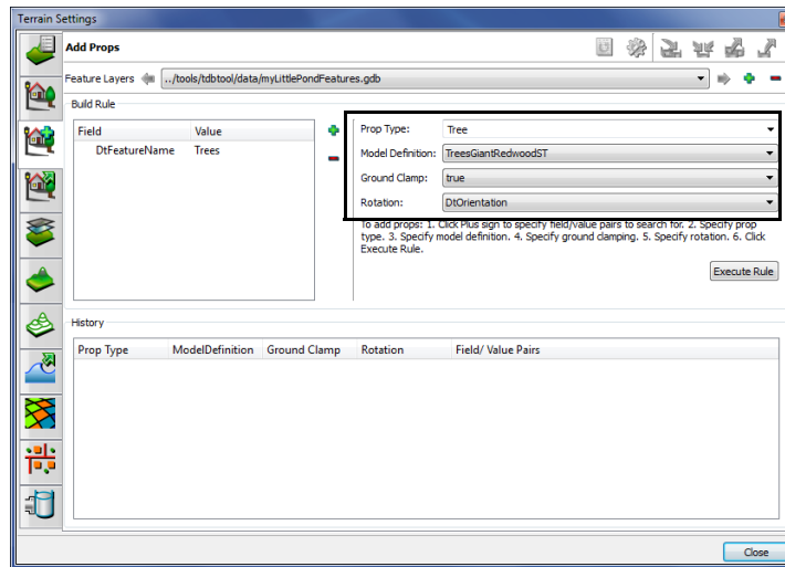
Figure 7-20. Full build rule specified
