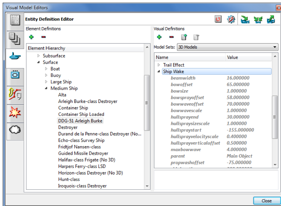
Figure 6-28. Ship Wake visual definition
