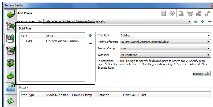
Figure 3-21. New Field/Value pair
