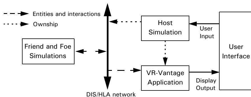
Figure 12-9. Networked IG Configuration
