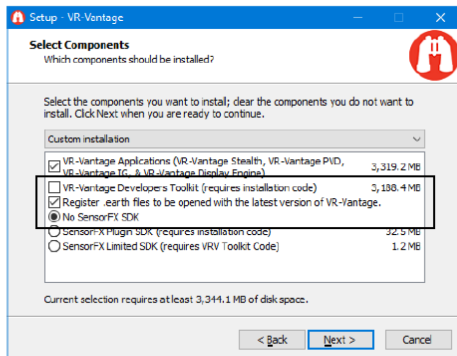
Figure 23. Installation wizard
