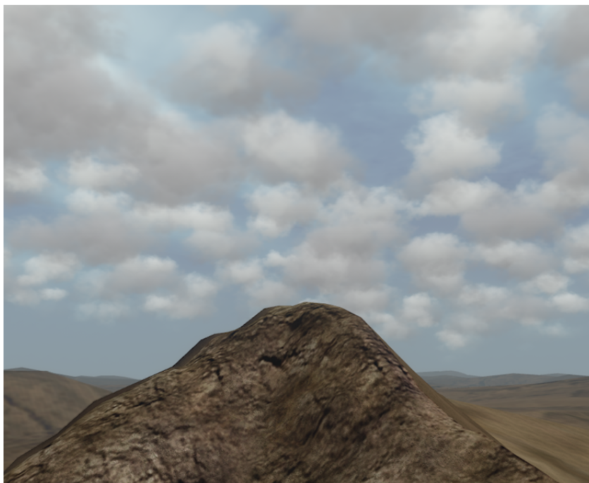
Figure 5. Cloud cover
