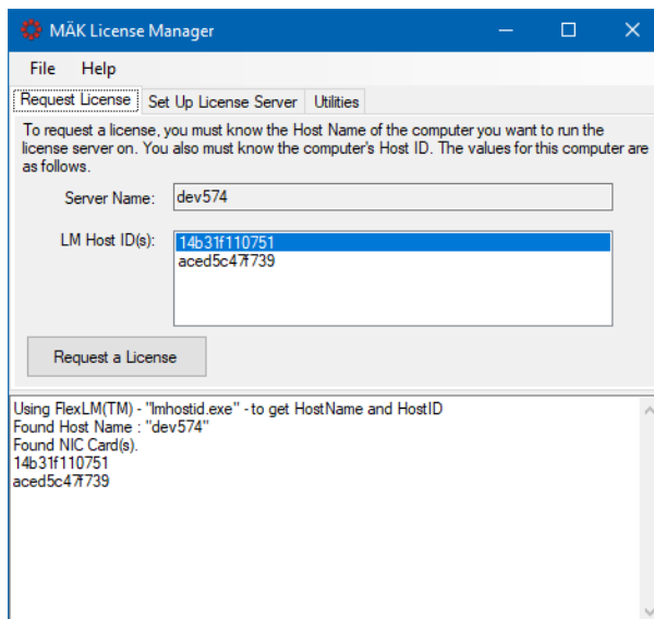
Figure 26. License Manager
