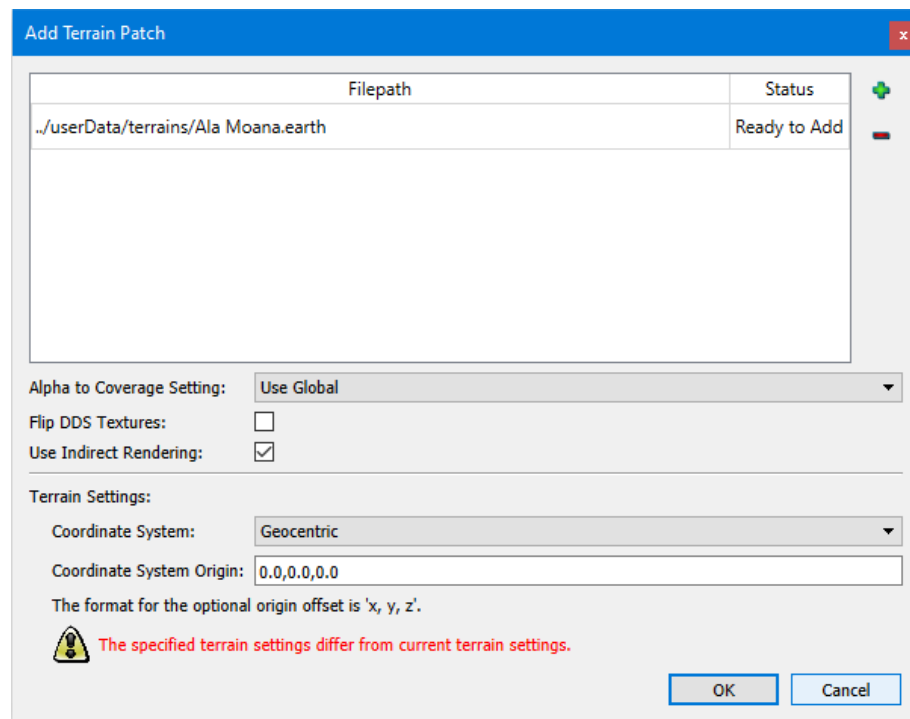
Figure 19. Add Terrain Patch
