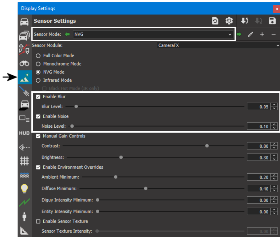
Figure 16. Sensor Settings
