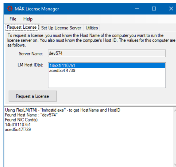
Figure 31. License Manager
