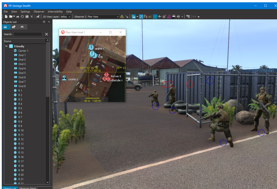
Figure 22. Raid demo
