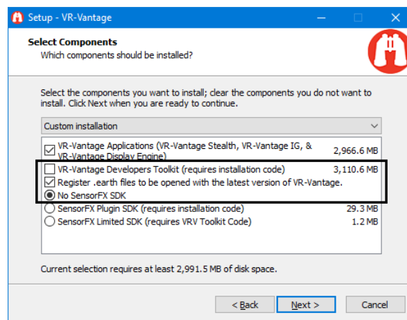
Figure 29. Installation wizard
