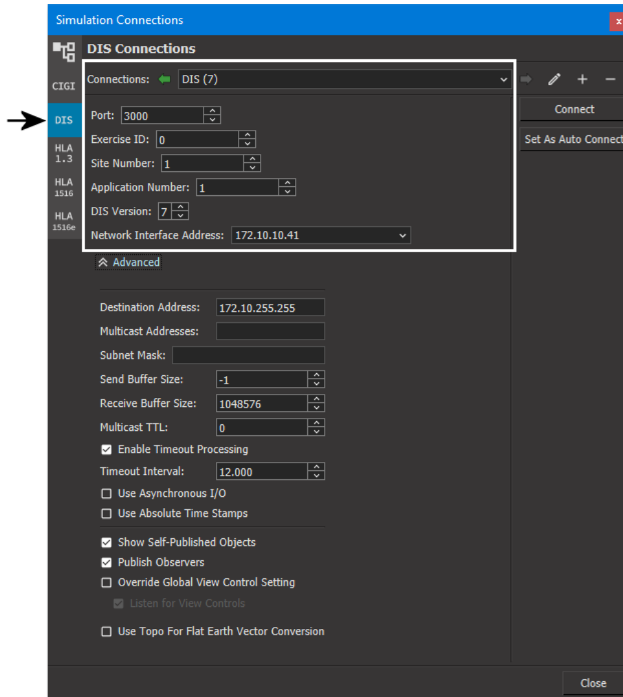
Figure 10. DIS Connection
