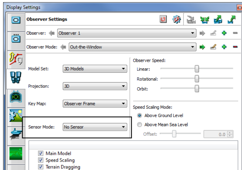
Figure 15. Sensor mode
