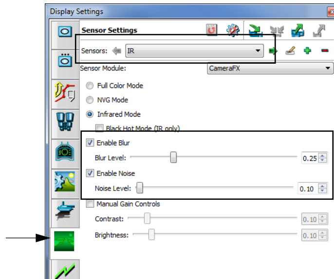
Figure 17. Sensor Settings
