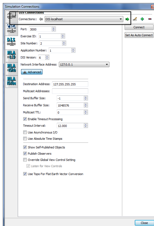
Figure 11. DIS Connection
