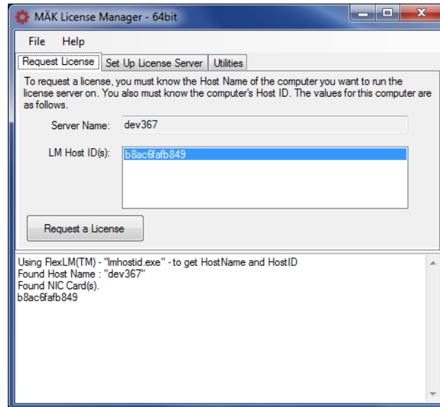
Figure 2-2. License Manager
