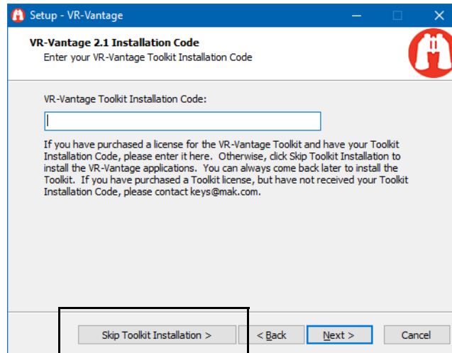
Figure 2-1. Installation wizard
