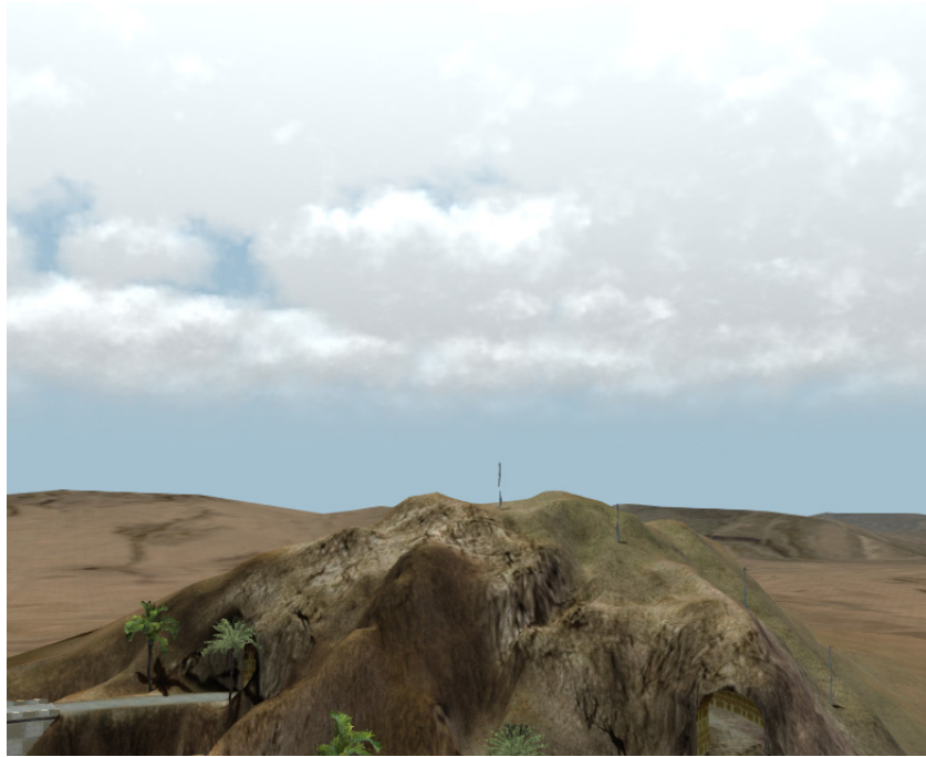
Figure 1-6. Cloud cover
