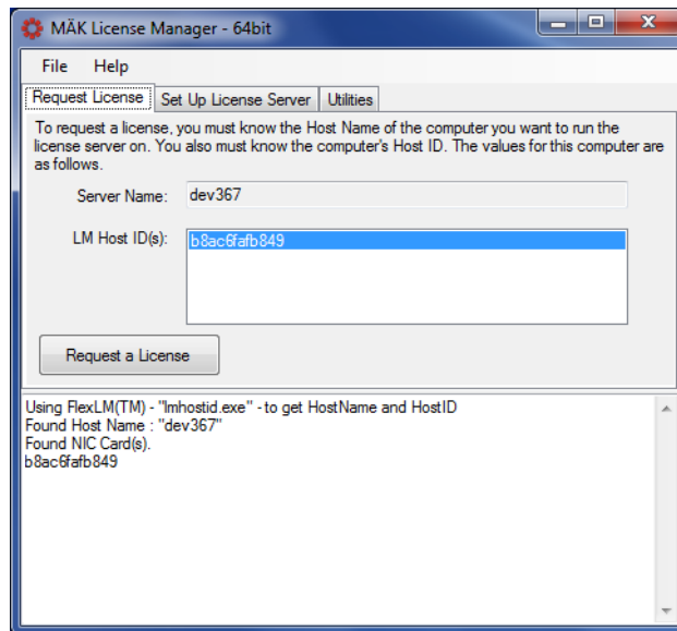
Figure 2-4. License Manager
