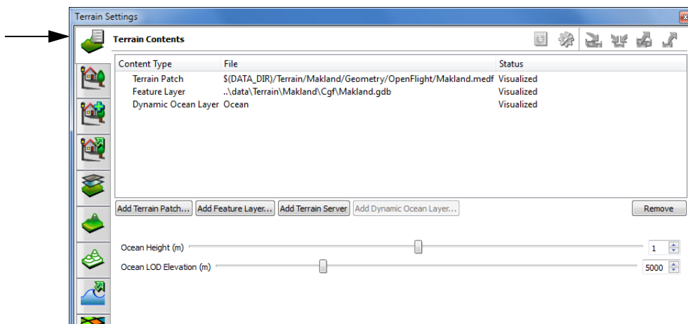
Figure 4. Terrain Contents
