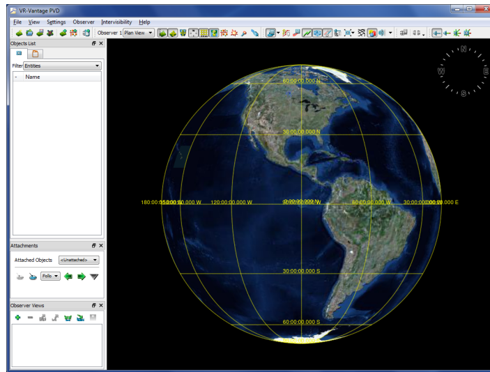
Figure 6. VR-TheWorldOnline
