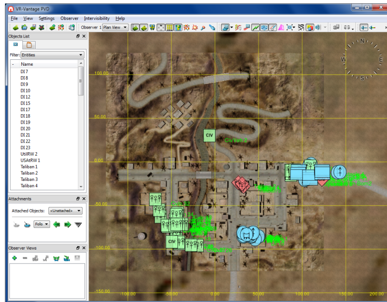
Figure 1. Simulation loaded
