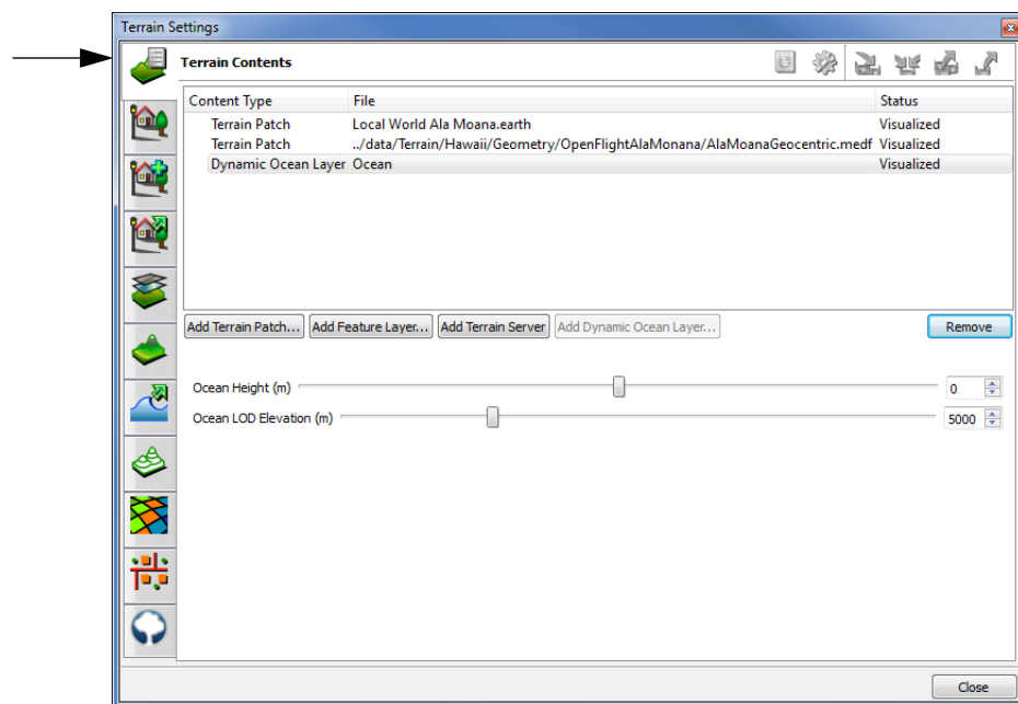
Figure 1-12. Terrain Contents
