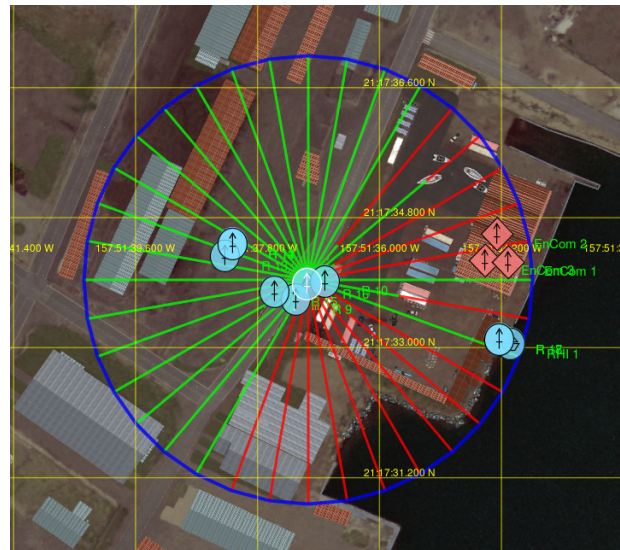
Figure 1-9. Intervisibility fan
