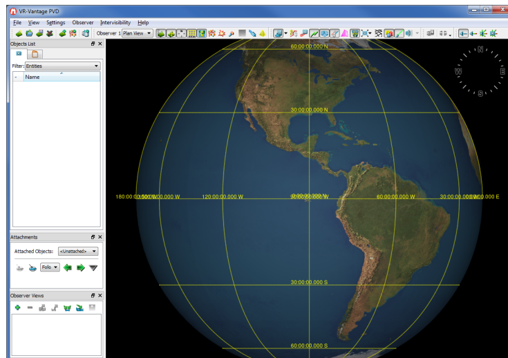
Figure 1-5. VR-TheWorld Online
