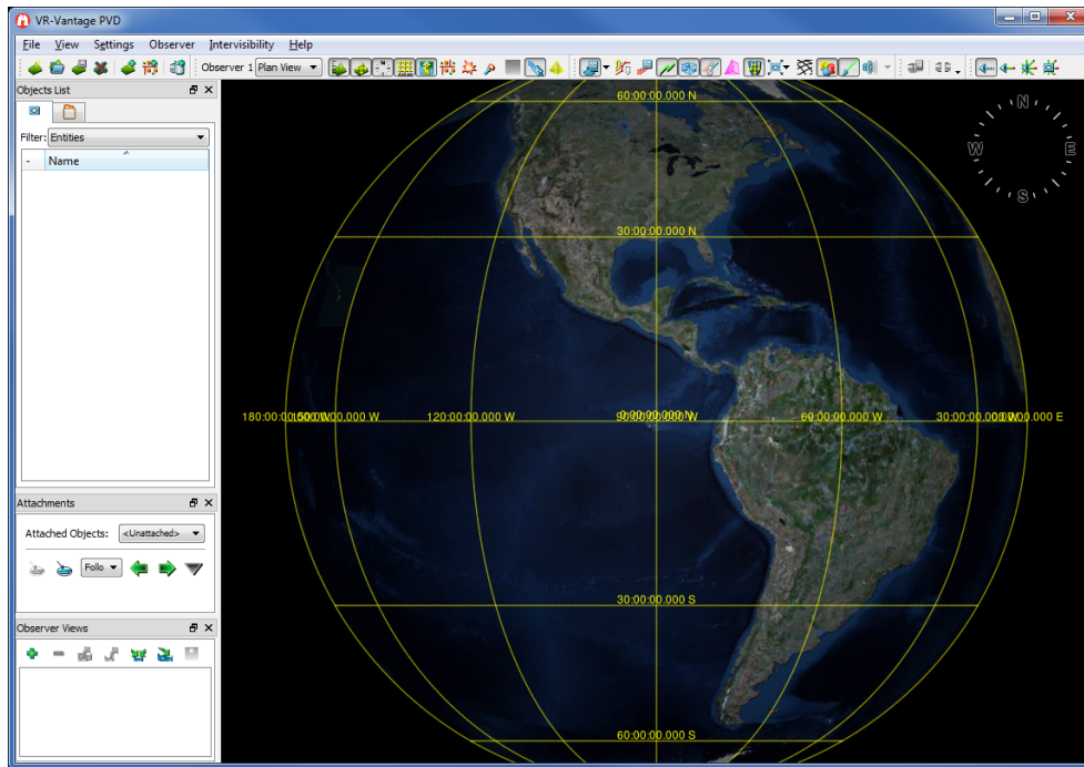
Figure 1-14. VR-theWorld Online
