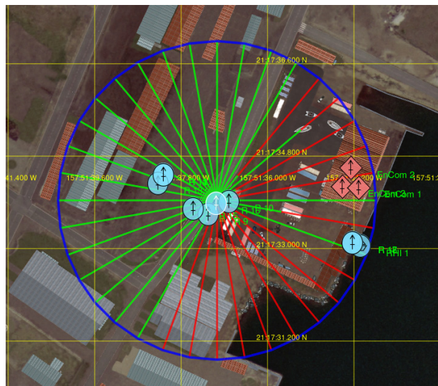
Figure 1-9. Intervisibility fan
