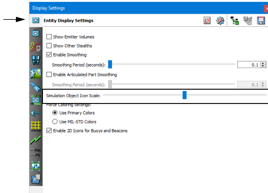
Figure 1-14. Entity Display Settings page
