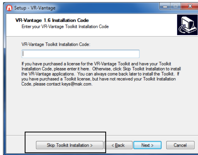
Figure 2-27. Installation wizard
