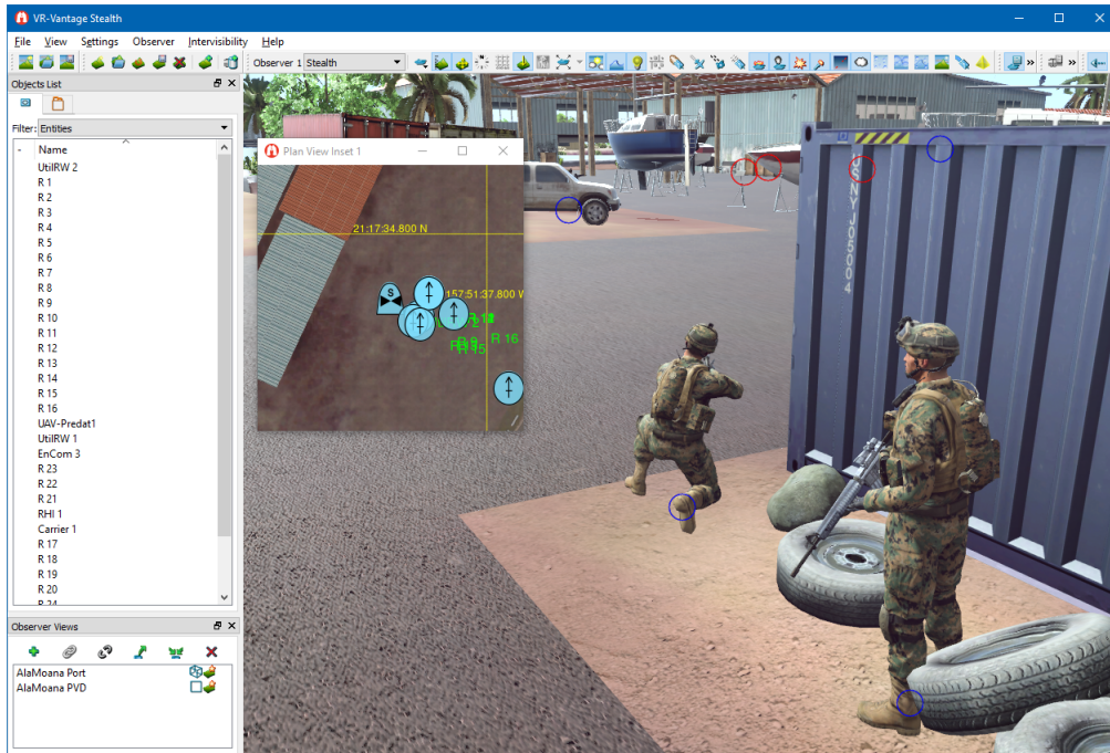
Figure 1-22. Raid demo
