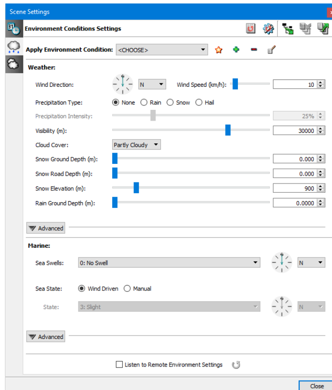
Figure 1-4. Scene Settings dialog box, Environment Conditions Settings page
